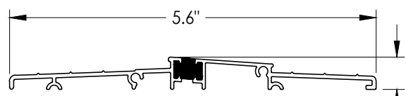
29 OUTSWING ADA THRESHOLD Endura (Z-Series)
