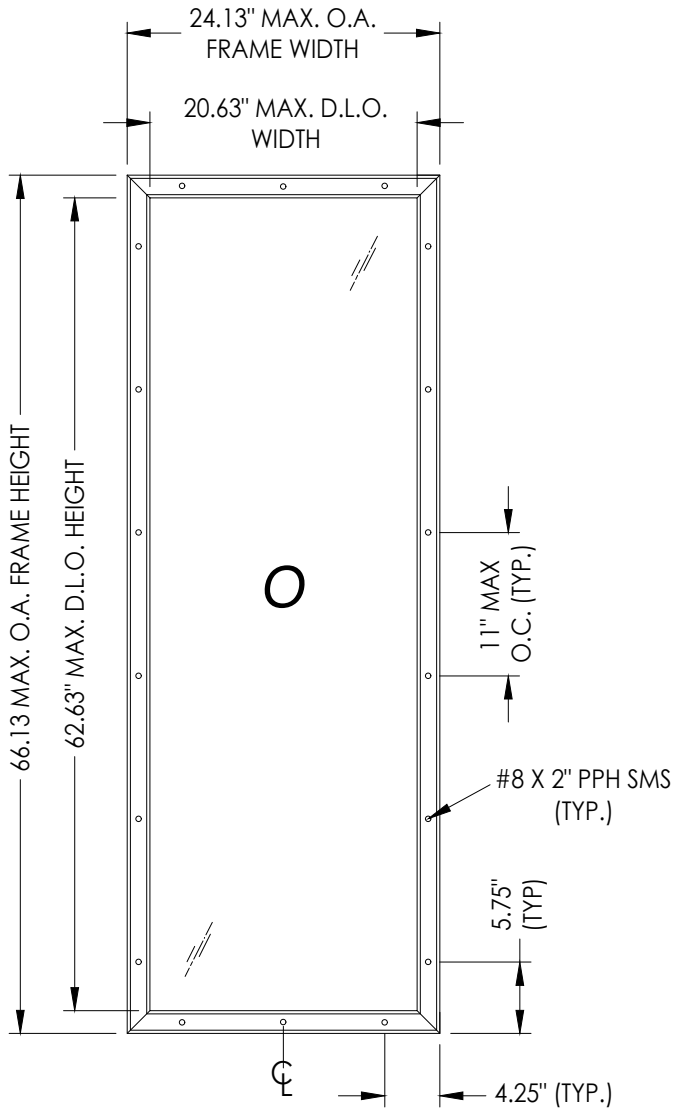
ODL LITE FRAME DETAIL "FLAT FRAME" PROFILE
