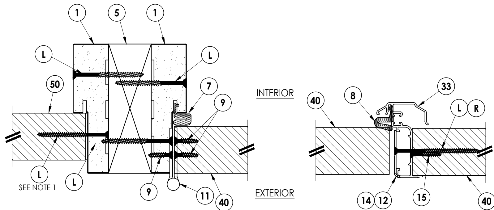
5 HORIZONTAL CROSS SECTION 5 Outswing shown (Inswing similar)
